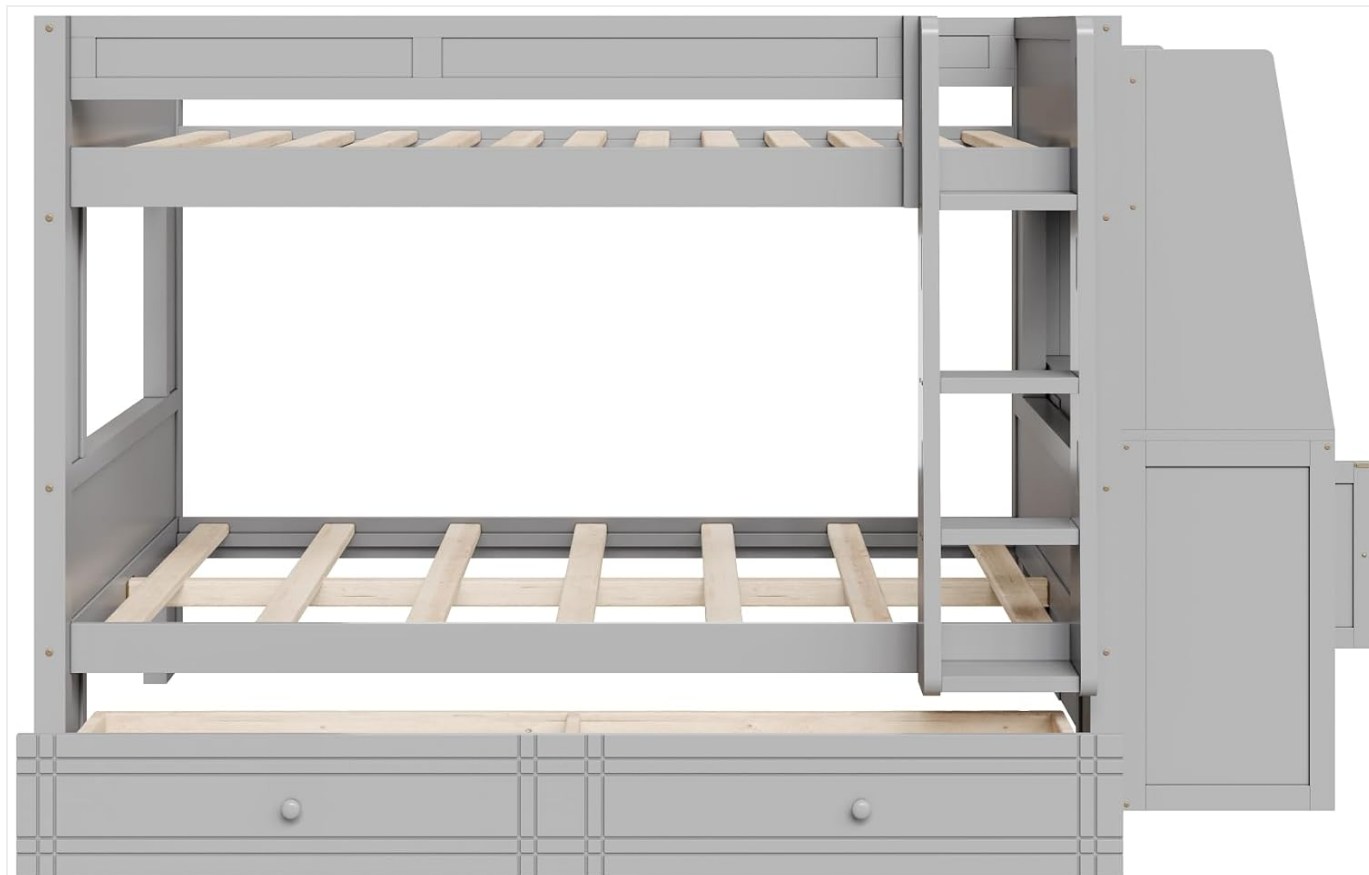
Image: Side view of the bunk bed frame, illustrating the slat support system.
