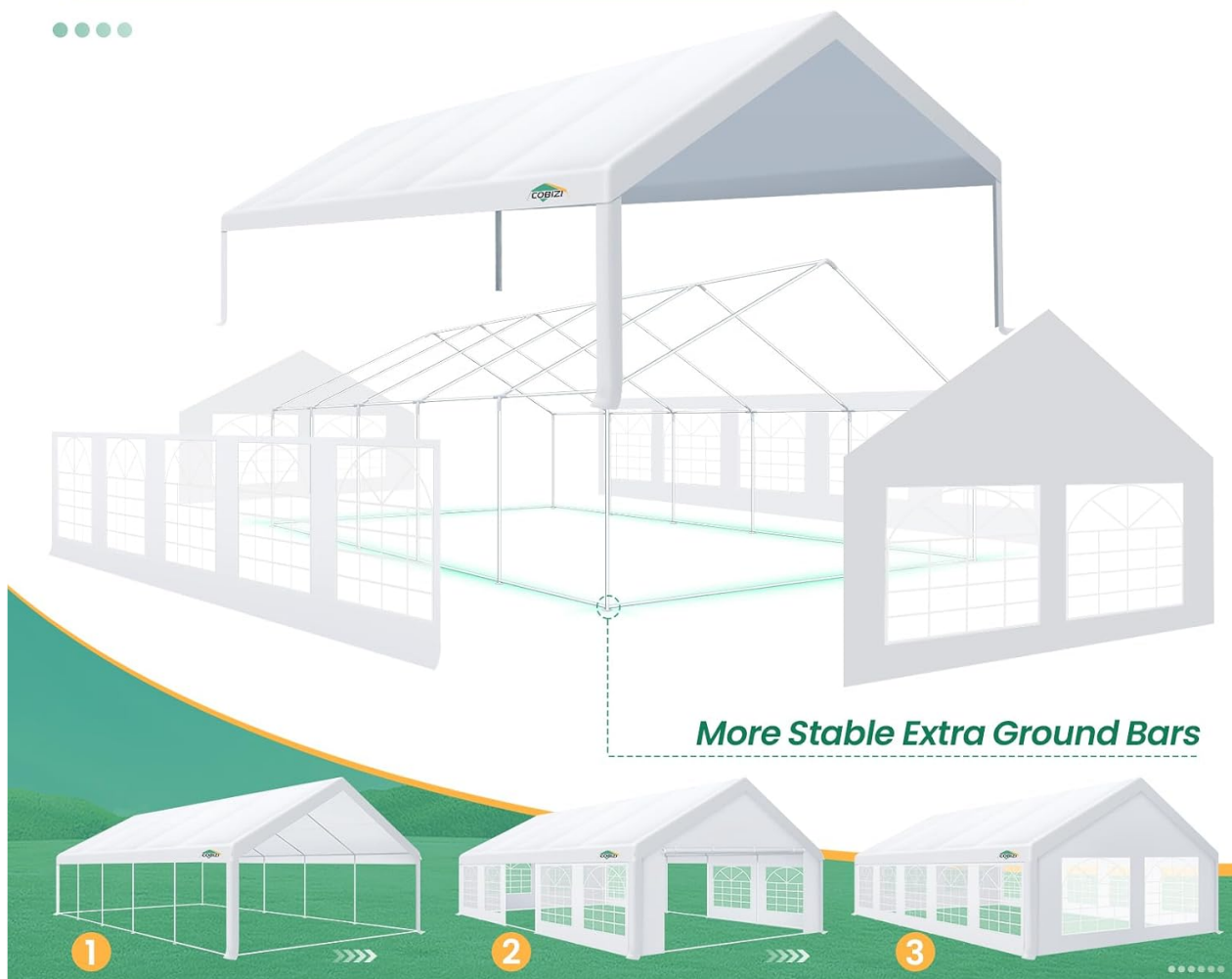
Visual guide for assembling the tent frame and attaching sidewalls.
