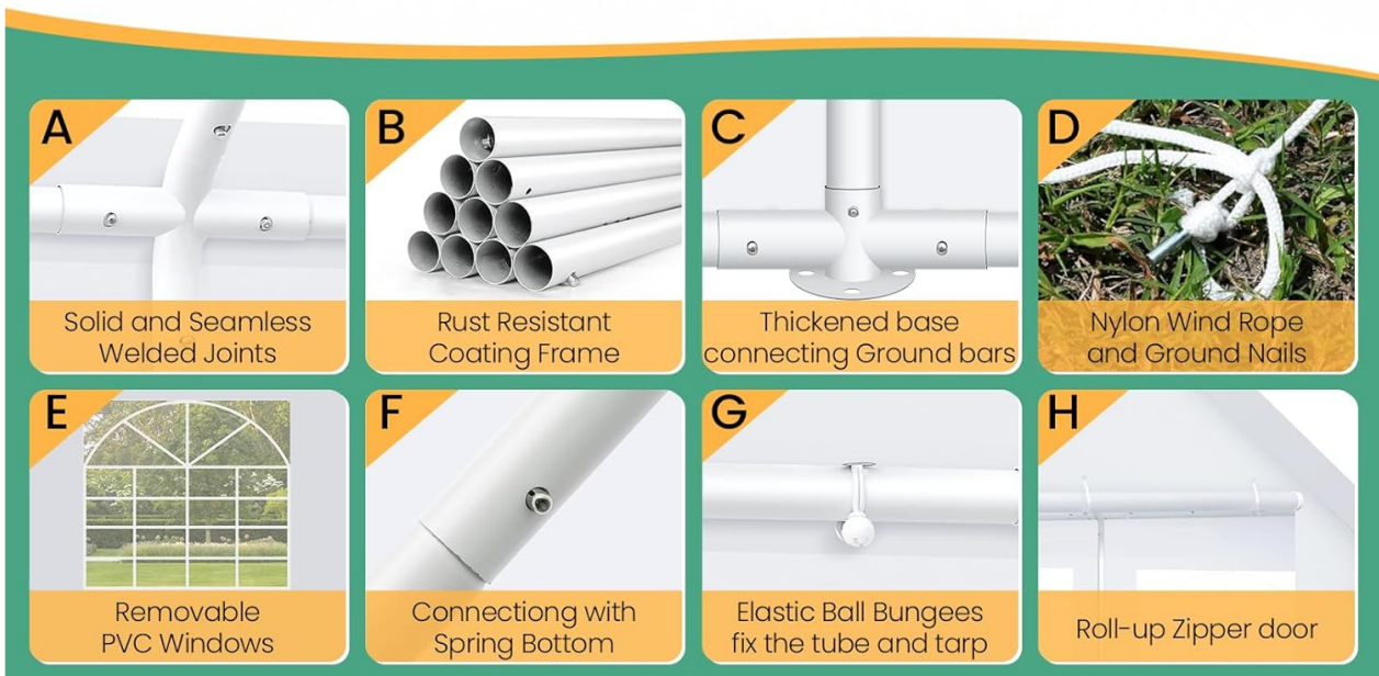
Key components of the tent structure and covering.
