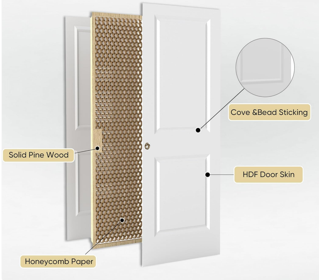
Image: Detailed view of the door panel construction, highlighting the HDF door skin, solid pine wood, and honeycomb paper core.
