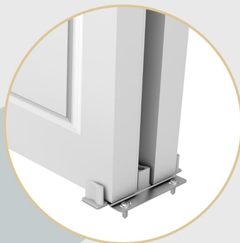
Figure 6: Details of the built-in front cover and floor guide.
