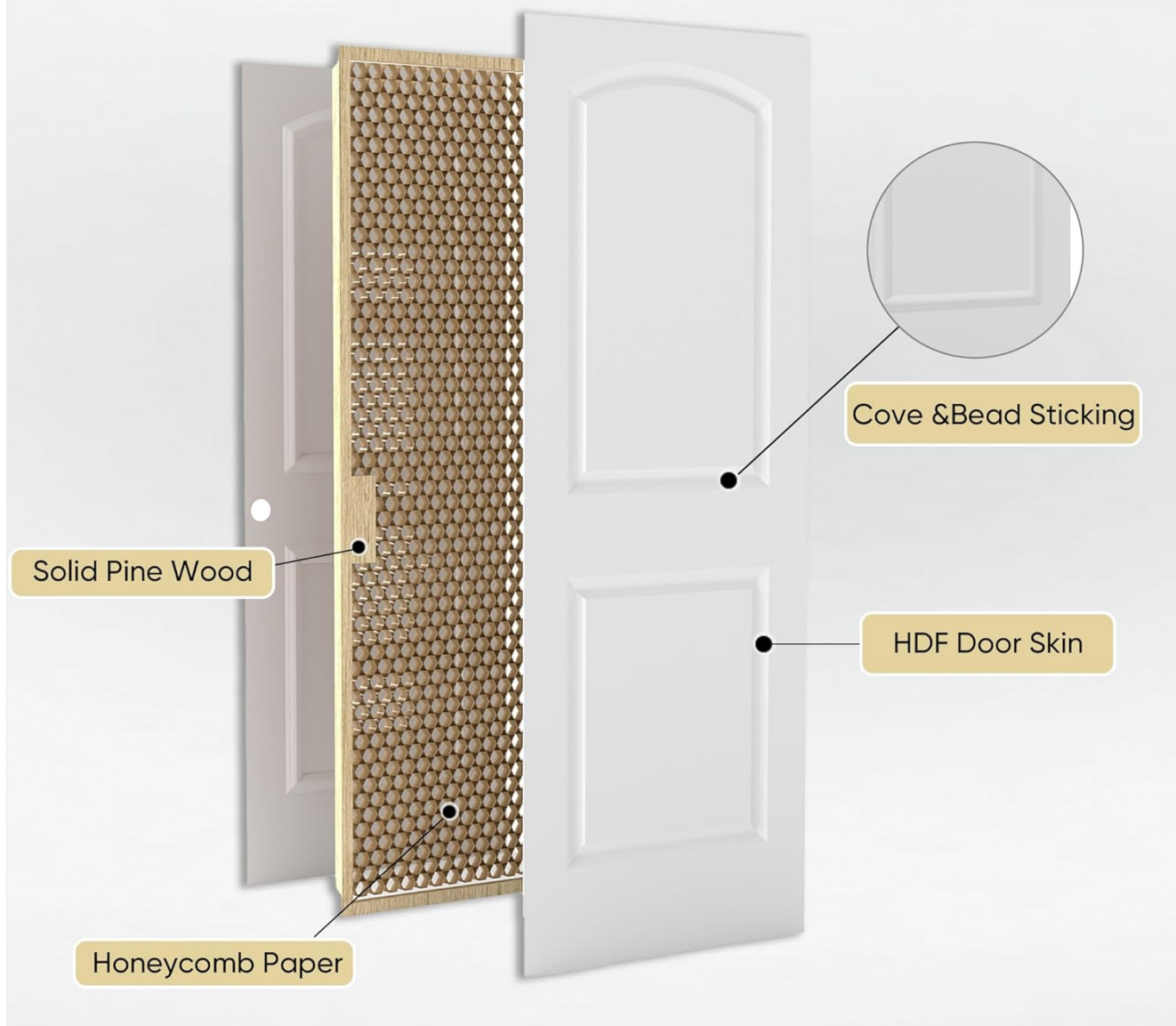
Figure 4: Door panel construction details.
