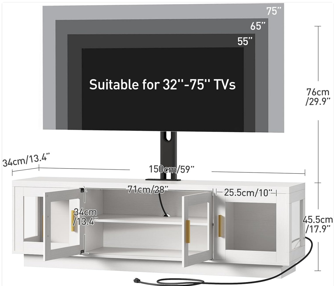
Image 8.1: Detailed dimensions of the TV stand and its compatibility with various TV sizes (32-75 inches).
