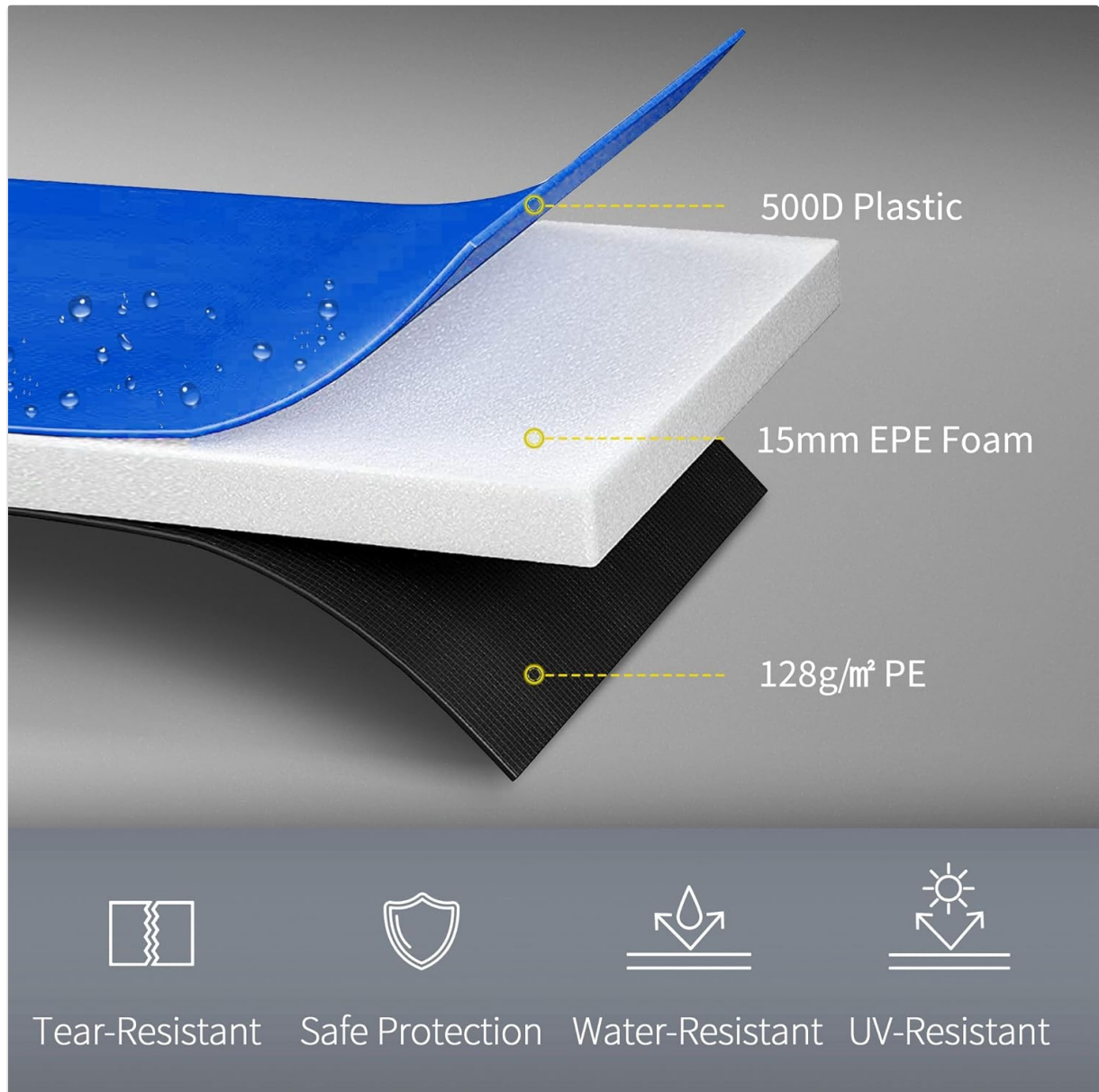
Image 3.2: Cross-section illustrating the material layers: 500D Plastic, 15mm EPE Foam, and 128g/m² PE, providing tear-resistance, safe protection, water-resistance, and UV-resistance.
