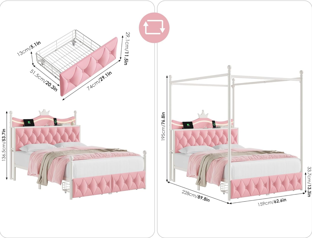
Figure 1: Bed frame dimensions and removable post configurations.
