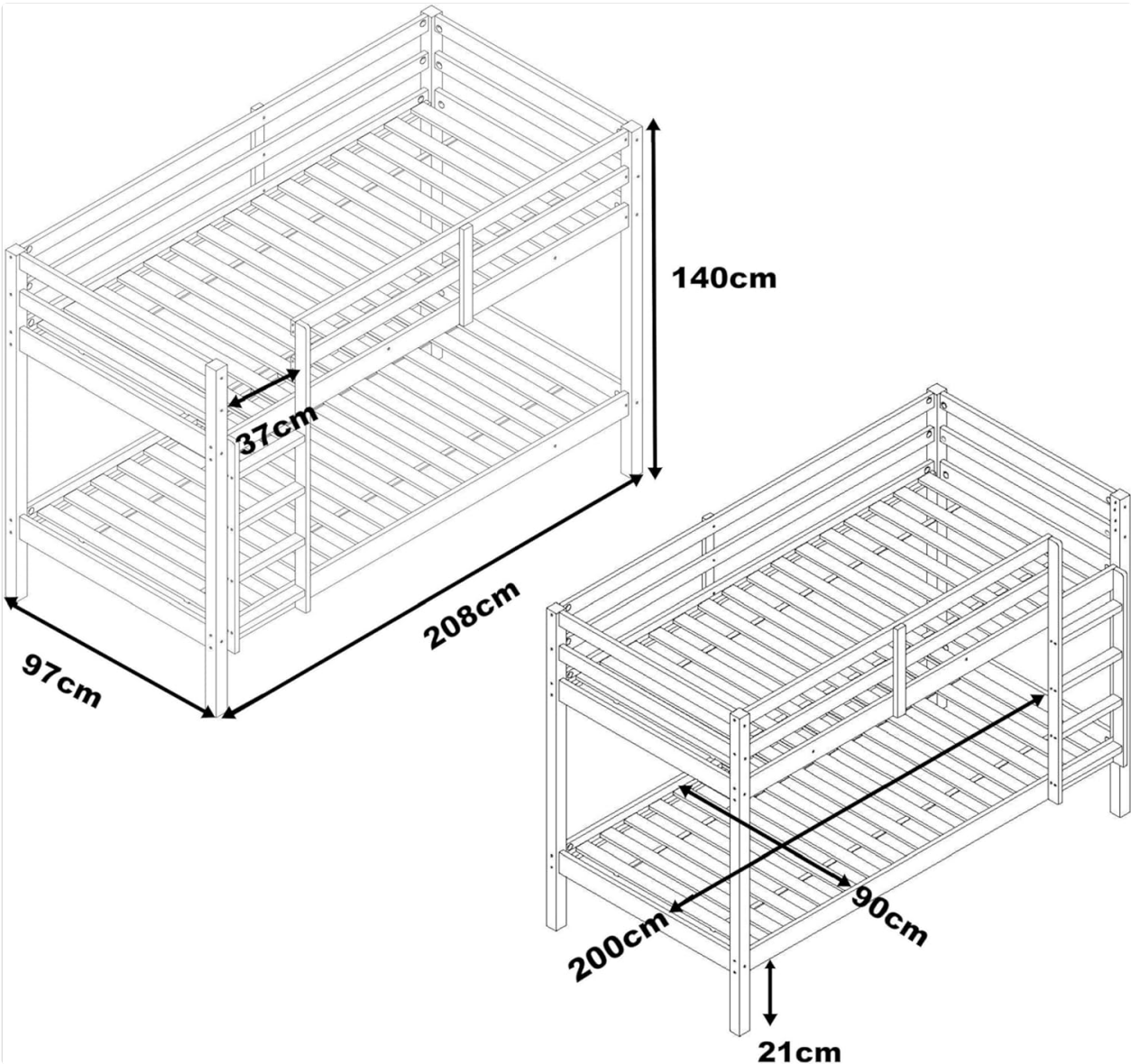
Image 7.1: Technical diagram illustrating the overall dimensions of the bunk bed, including length (208 cm), width (97 cm), and height (140 cm), as well as internal mattress dimensions and ladder width.
