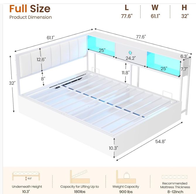
Figure 4.2.2: Product Dimensions. This diagram provides the overall measurements of the assembled bed frame.
