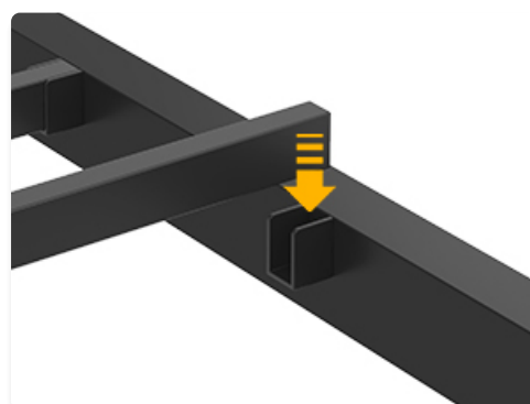
Figure 4: Buckle design for easy installation of the metal slats.
