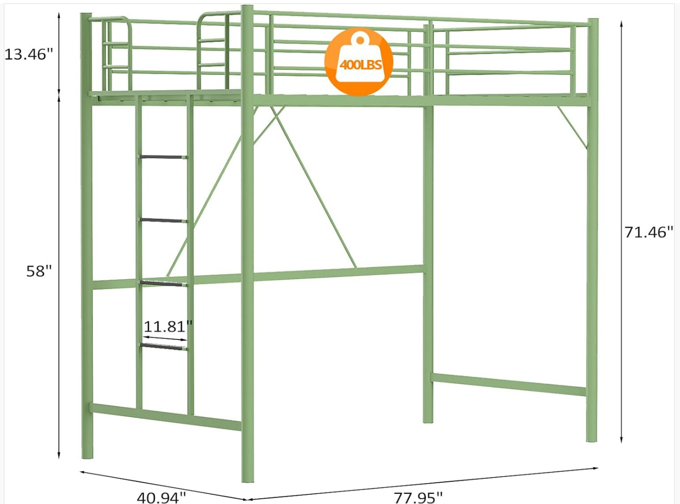
Image: Detailed dimensions of the VINGLI Twin Size Loft Bed.
