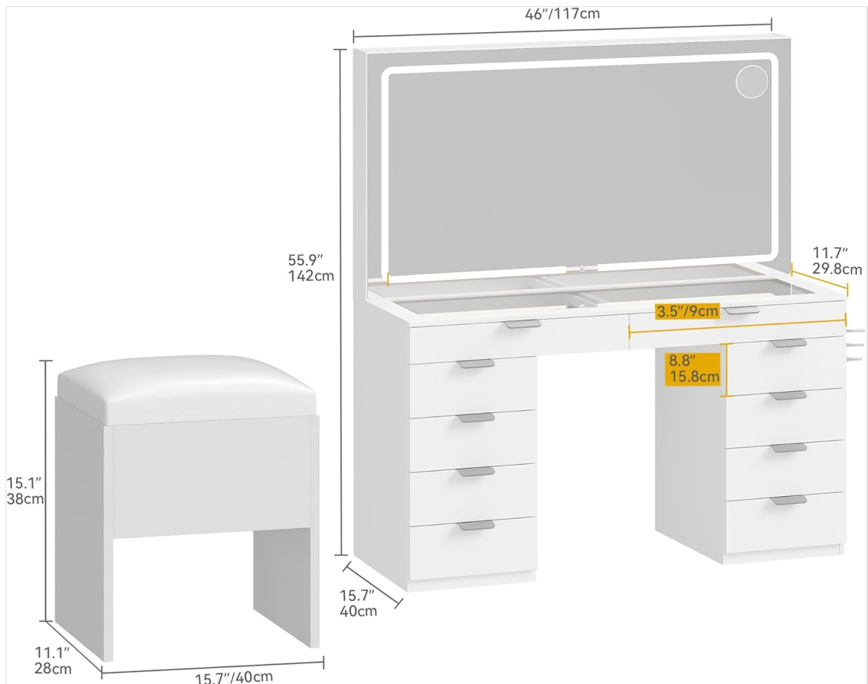
Figure 1: Dimensional diagram of the DWVO Vanity Desk and accompanying stool. The desk measures 46 inches wide, 15.7 inches deep, and 55.9 inches high including the mirror. The stool measures 15.7 inches wide, 11.1 inches deep, and 15.1 inches high.
