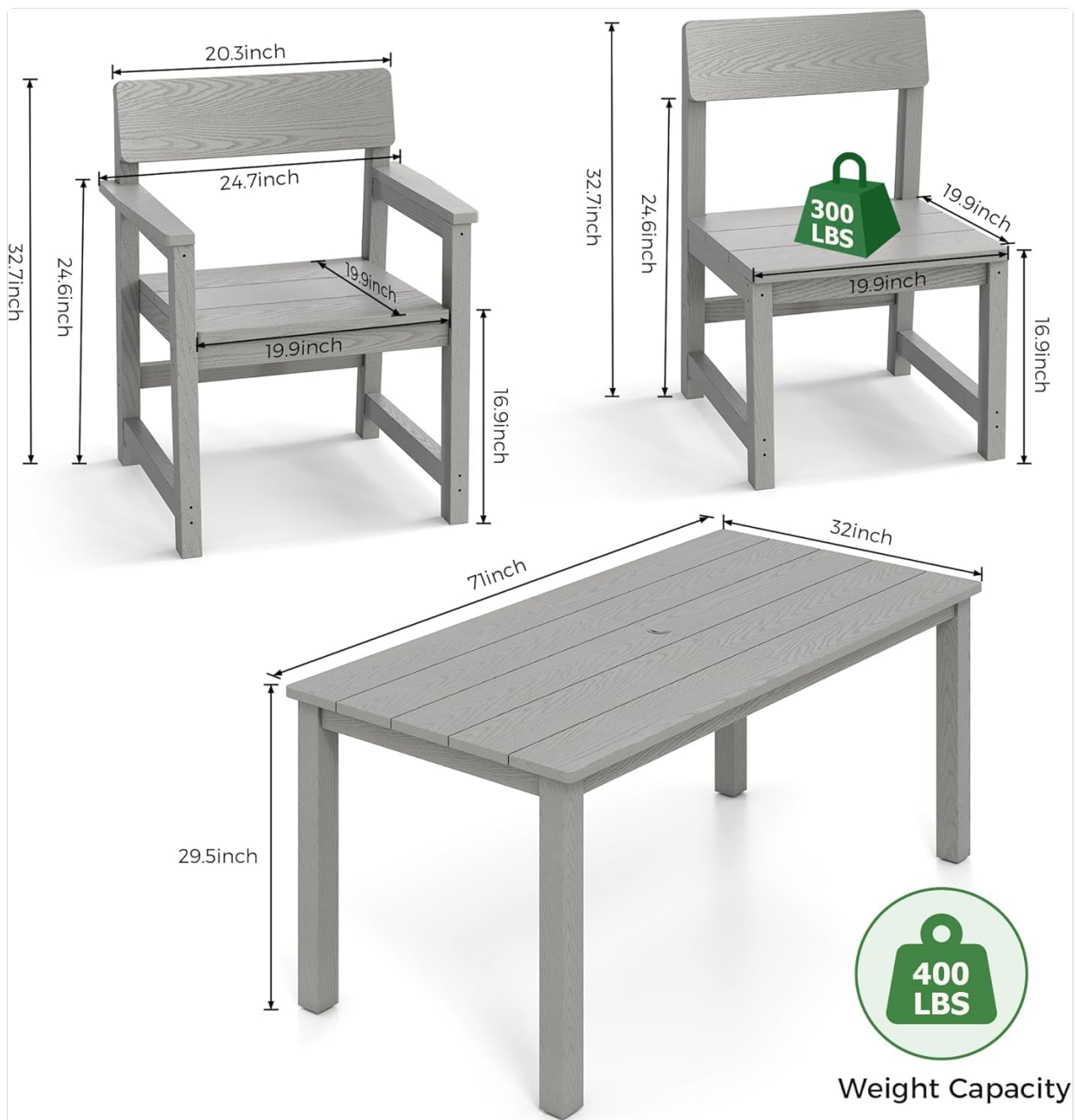
Image: Detailed dimensions and weight capacities for the dining table, armchair, and armless chair components.
