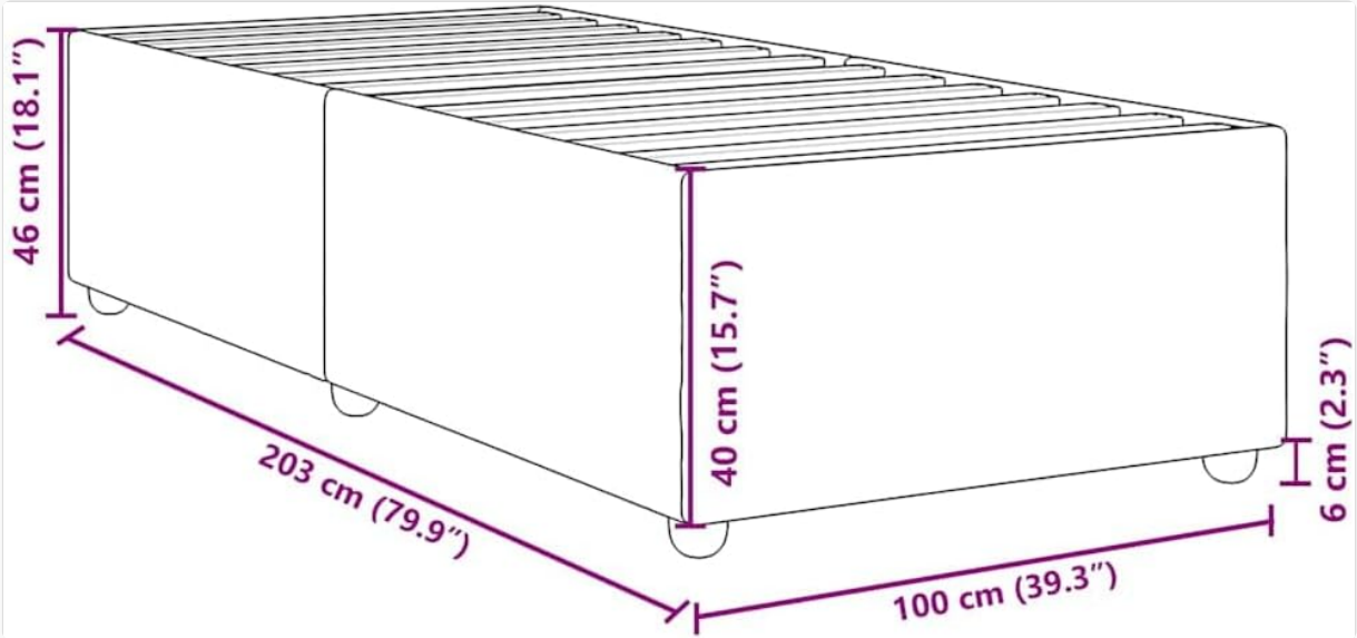
Image: Dimensional diagram of the bed frame, indicating width, length, and height measurements.
