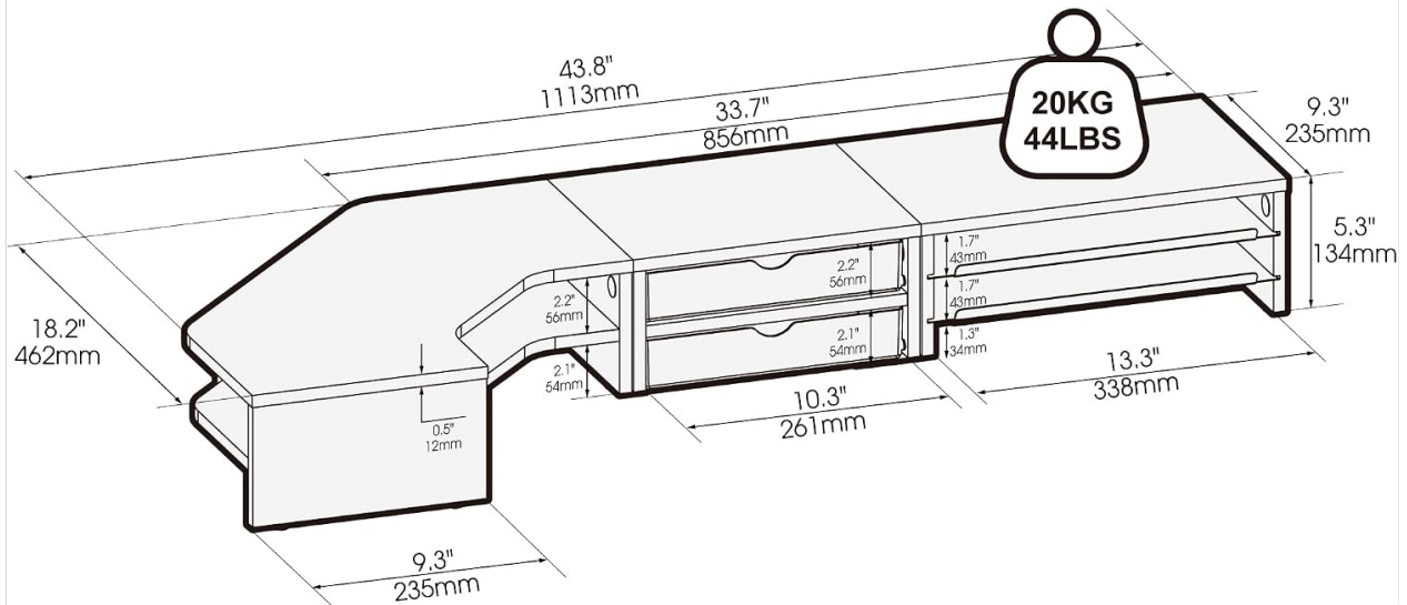
Figure 4.4.3: Example of a straight, extended assembly style for multiple devices.
