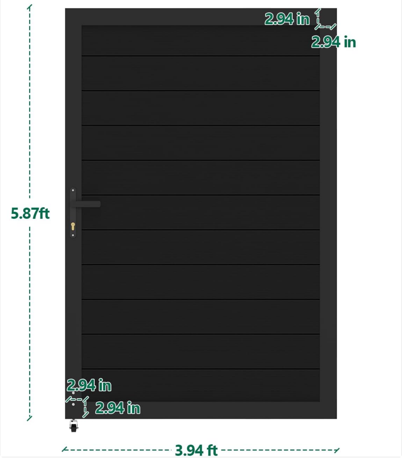
Image: A diagram illustrating the precise dimensions of the Treslam Privacy Gate, including its height (5.87ft or 70.44 inches) and width (3.94ft or 47.28 inches), along with frame thickness details.
