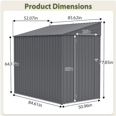
Detailed diagram showing the dimensions of the shed, including roof overhangs and door opening size.
