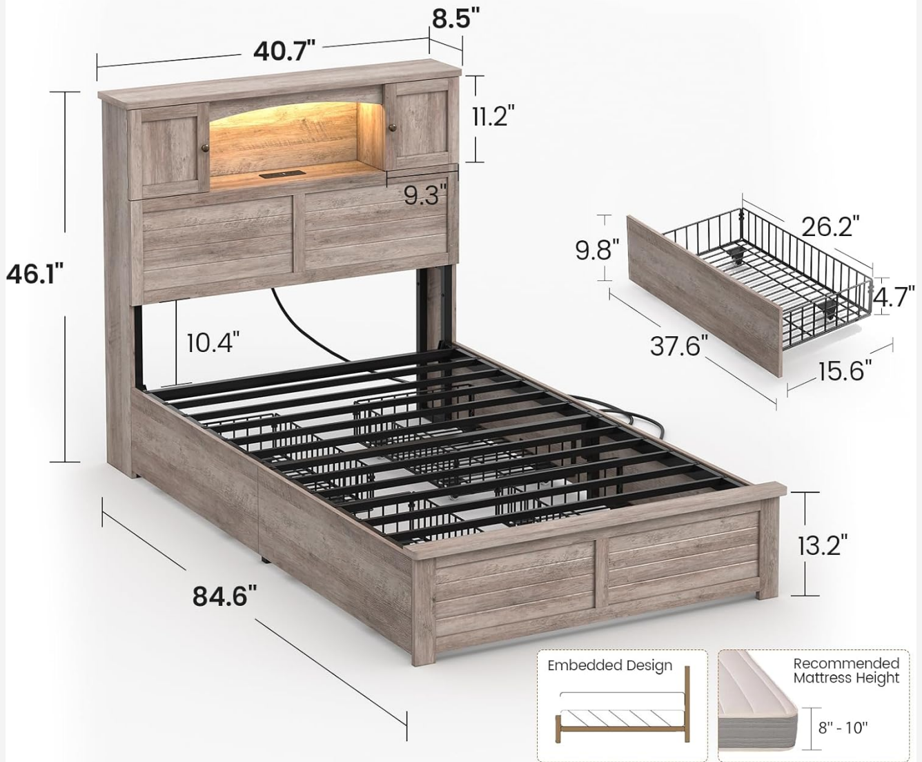
Image: Detailed dimensions of the MSmask Twin Bed Frame, including headboard height, frame length, and drawer size.
