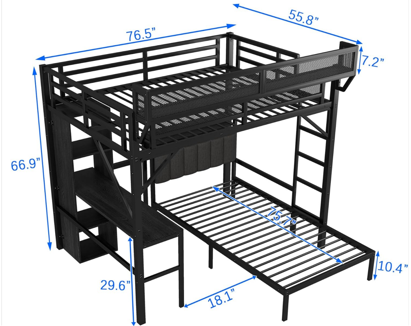
Image 7.1: Diagram illustrating the key dimensions of the SOFTSEA Full Over Twin Bunk Bed.
