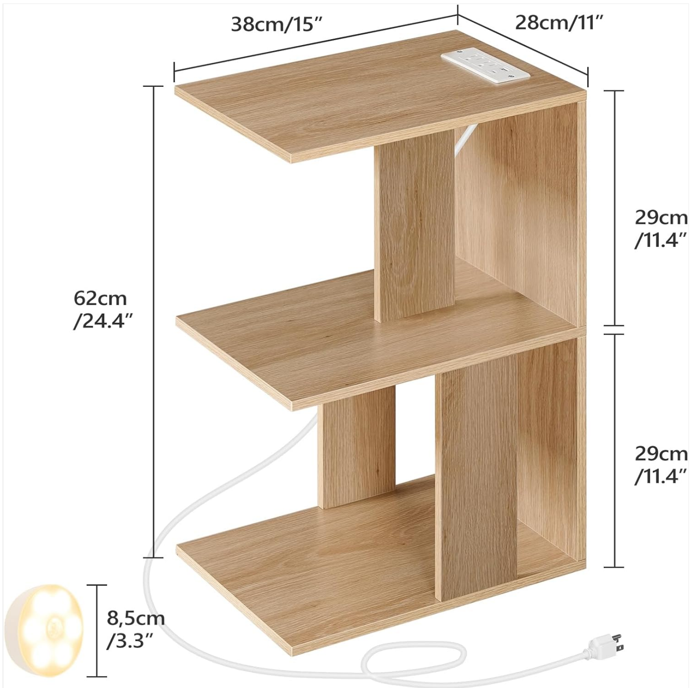
Figure 7.1: Product Dimensions.
