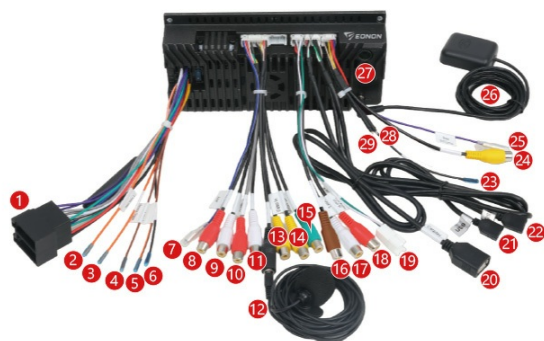
Image 4.3: Eonon UX7-PLUS wiring diagram with labeled ports.
