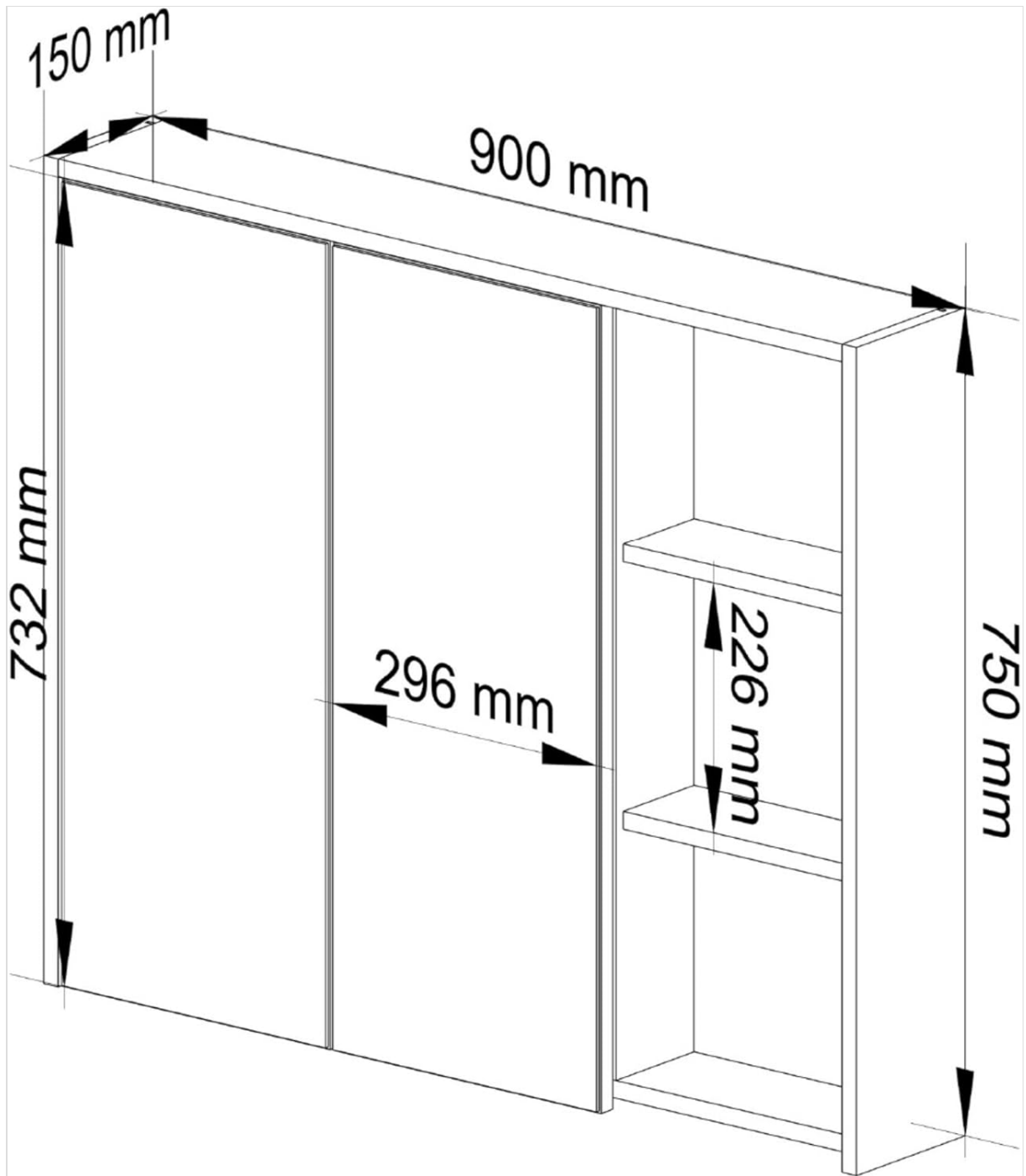
Figure 1: Cabinet Dimensions (Width: 900mm, Height: 750mm, Depth: 150mm)
