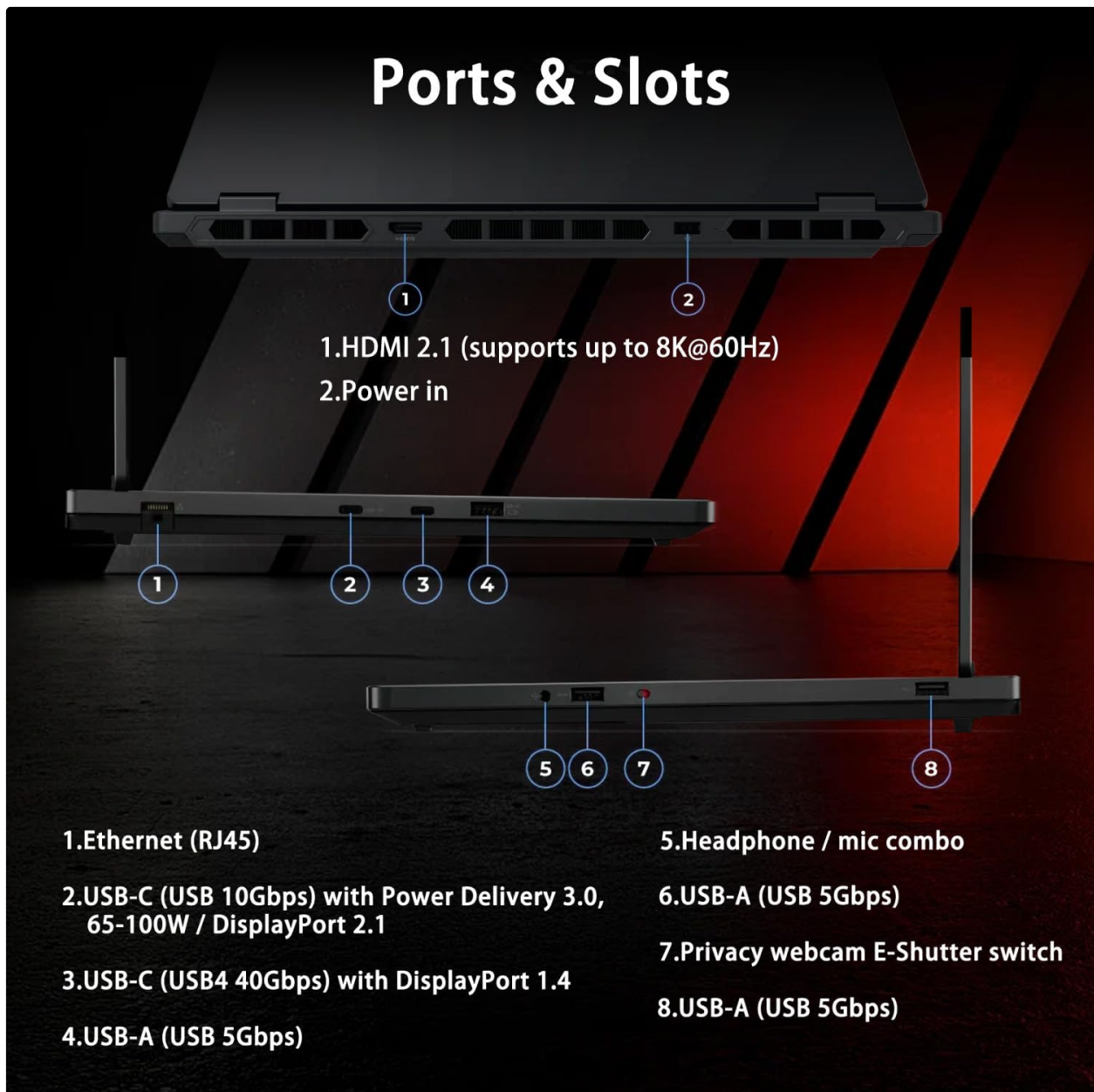
Image: Detailed diagram illustrating the location and type of all ports and slots on the Lenovo Legion 5 15AHP10 laptop, including HDMI, Power, Ethernet, USB-C, USB-A, and headphone/mic combo jack.
