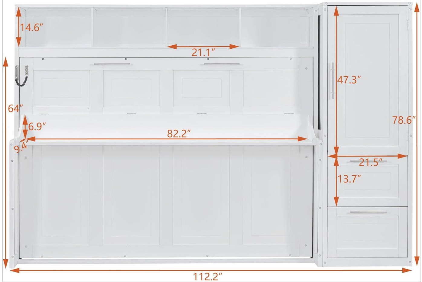
Figure 2: Closed Configuration Dimensions. This diagram provides the measurements of the Murphy bed when folded and stored within its cabinet, emphasizing its space-saving design.
