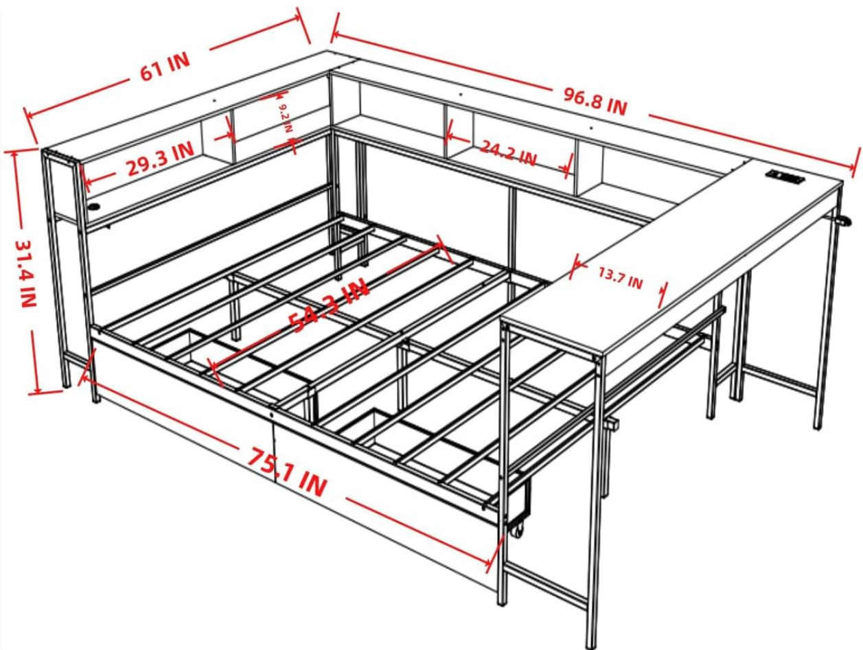
Image 3.1: Detailed dimensions diagram of the bed frame, illustrating overall length, width, and height of the bed, desk, and storage components.
