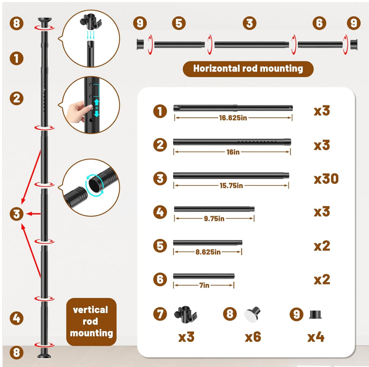
Figure 1: Detailed diagram of all included components for assembly.
