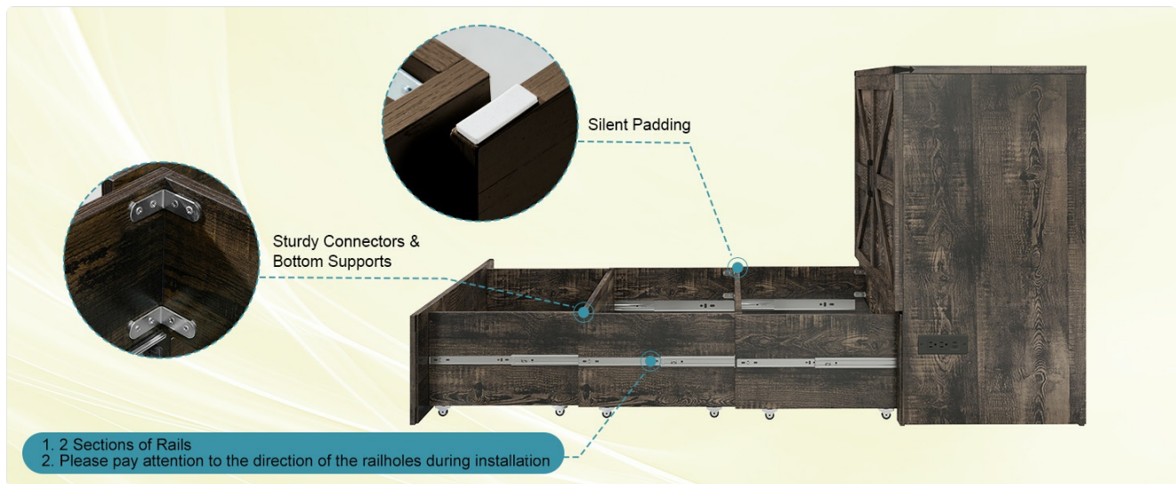
Image: Details of sturdy connectors, silent padding, and drawer rail installation.
