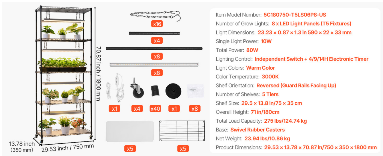
Image: Detailed diagram of all components included in the VEVOR plant shelf package.
