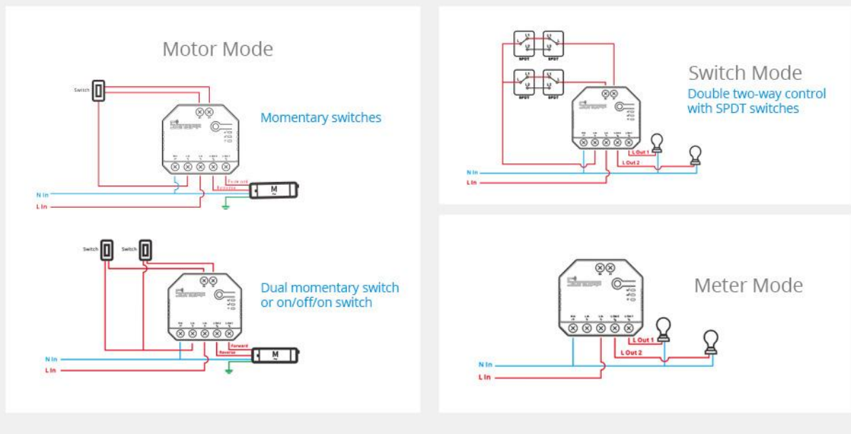
Figure 5.1: This diagram illustrates the various wiring configurations for the DUALR3 in Motor Mode, Switch Mode, and Meter Mode.
