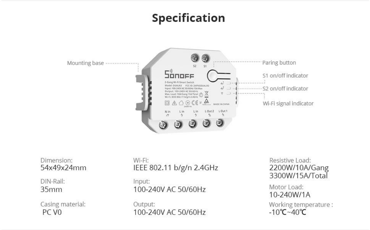
Figure 9.1: An annotated diagram of the DUALR3 showing its dimensions, buttons, indicators, and key technical specifications.
