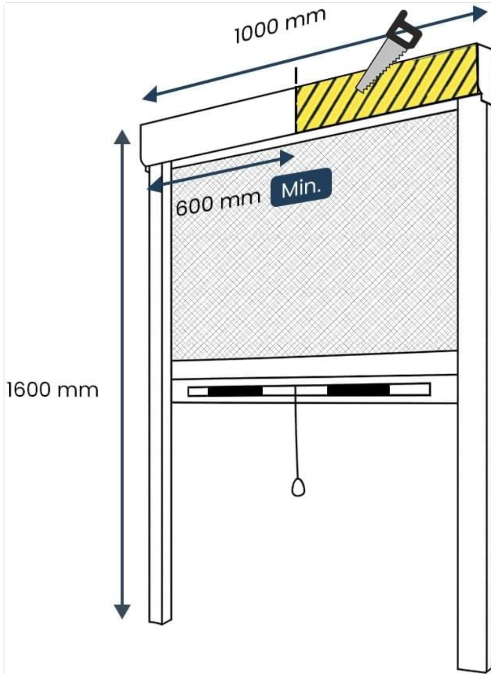
Figure 4: Guide for cutting the screen to your window's dimensions. Note the minimum width of 600mm.
