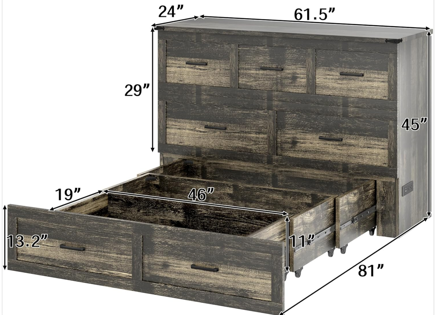
Image 8.1: Product dimensions for the roomfitters Murphy Bed Cabinet.
