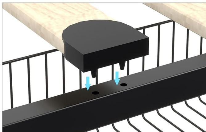
Figure 2: Details of the bed frame's support system, including metal and wood slats, EVA mute sponge, and the snap-on slat design for easy assembly.
