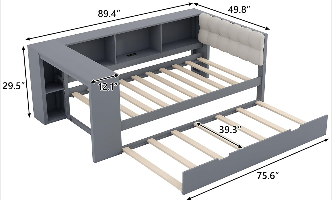
Image 3.1: Product dimensions for planning placement. Main bed: 89.4"L x 49.8"W x 29.5"H. Trundle: 75.6"L x 39.3"W.
