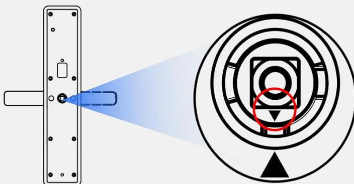
Figure 5: Important installation note: The arrow on the smart lock panel must point downwards.
