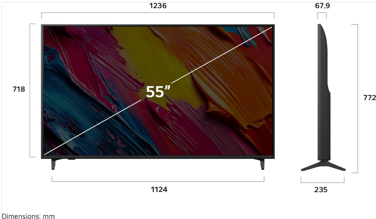
Figure 1: Front view of the LG 55QNE70A6A Smart TV.
