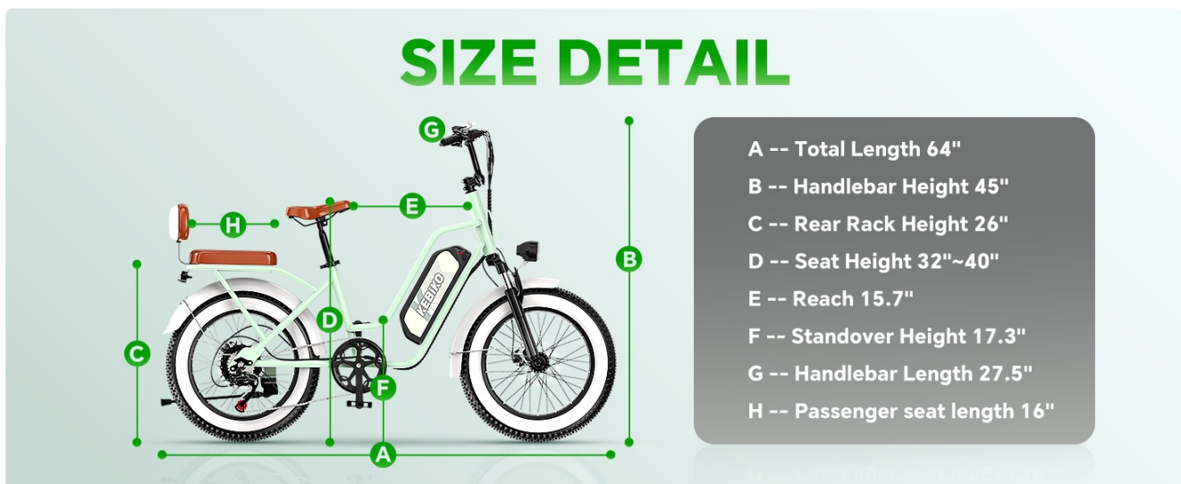
Image 8.1: Detailed diagram showing the dimensions of the bluebiko F8P electric bike.
