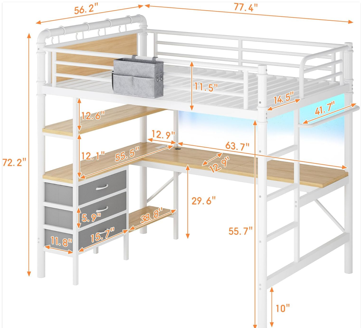
Figure 2: Overall Dimensions. This image provides a detailed view of the loft bed's dimensions, including height, width, and length, as well as desk and shelf measurements.
