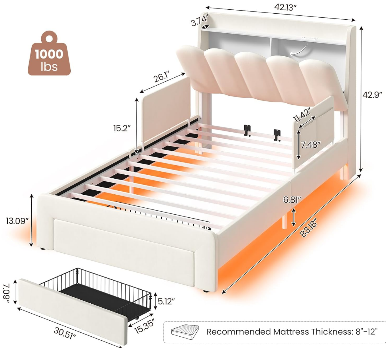
Figure 2: Product Dimensions and Weight Capacity
