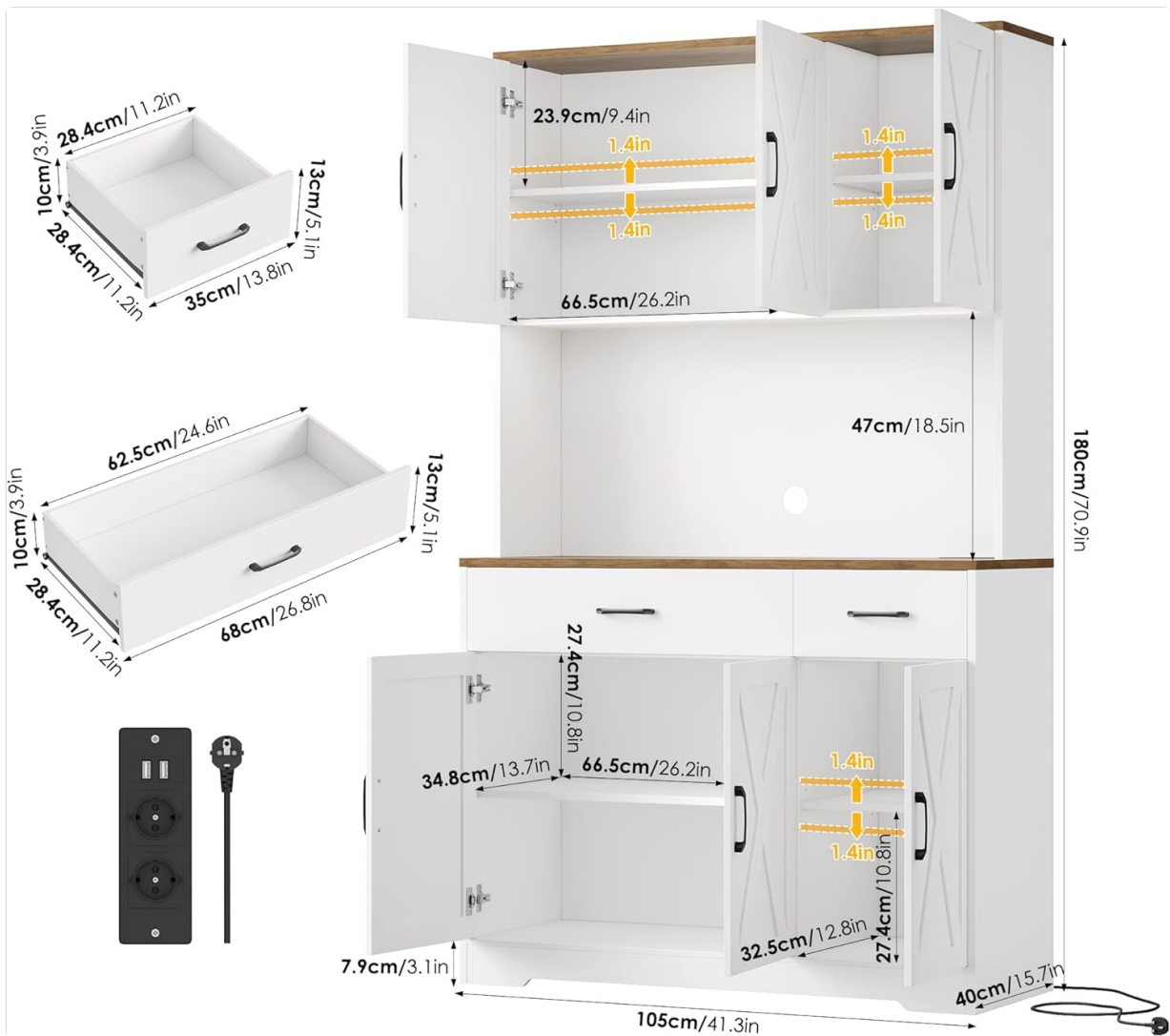
Image 1: Cabinet dimensions and structural overview. This diagram illustrates the various measurements of the cabinet, including the height of the upper and lower sections, the width of the worktop, and the depth of the unit. It also shows the internal layout with adjustable shelves and drawer sizes.
