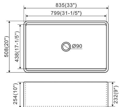
Figure 3: Kitchen sink dimensions and garbage disposal compatibility.
