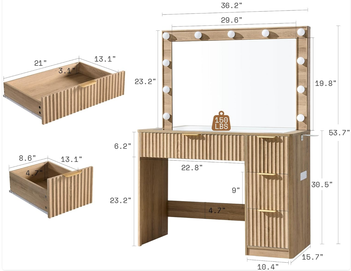
Figure 2: Detailed dimensions of the AMERLIFE 36.2" Fluted Vanity Desk, including drawer sizes and overall height.
