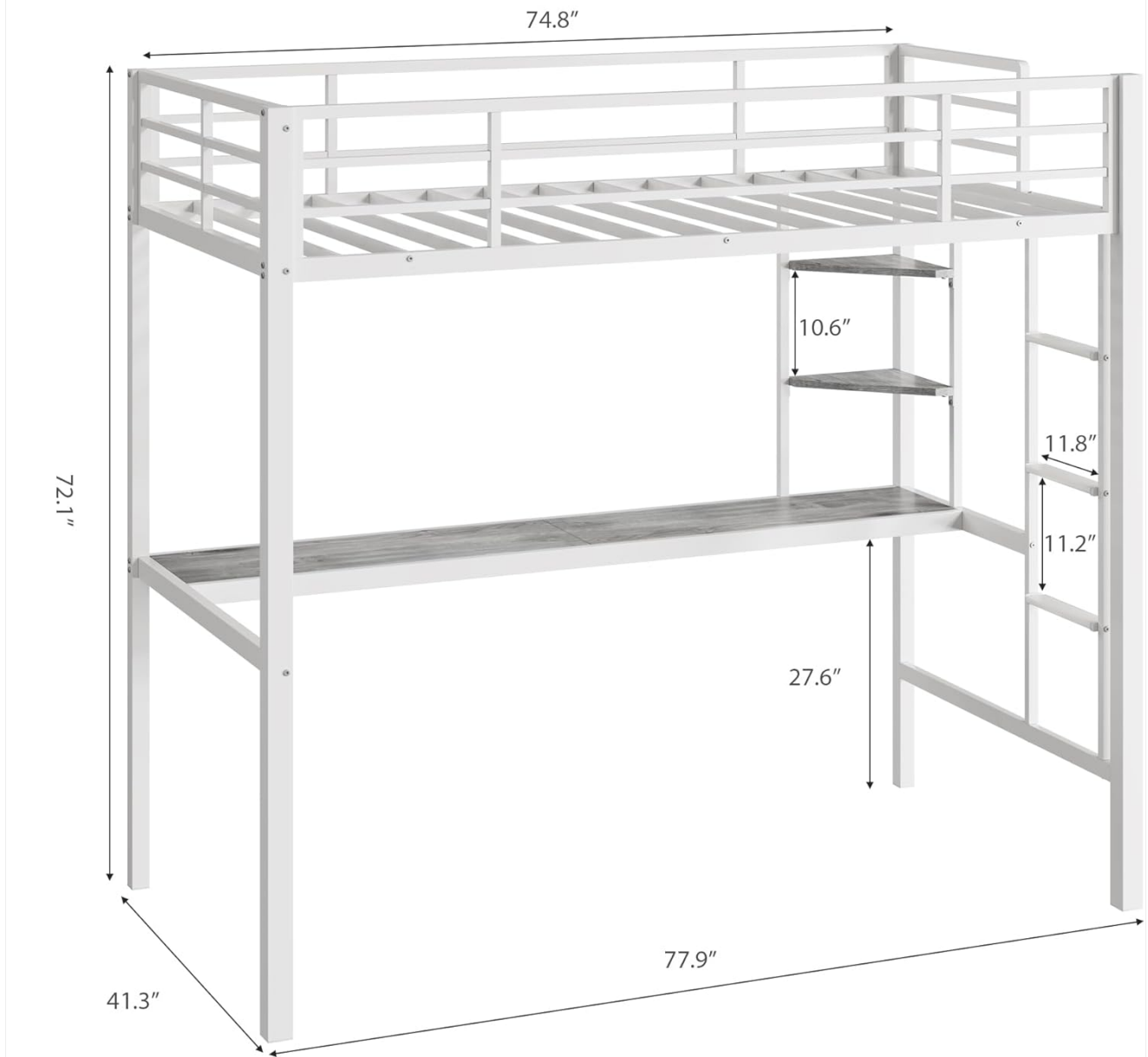
Image: Product dimensions diagram for the Garvee Twin Size Loft Bed.
