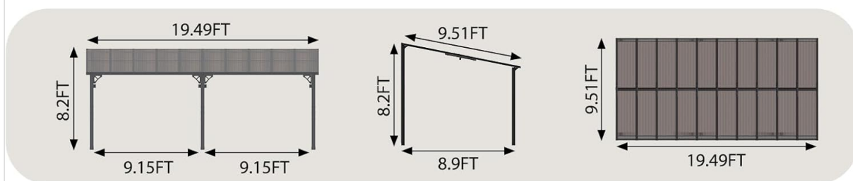
Figure 6: Product dimensions for the 10ft x 20ft hardtop gazebo.
