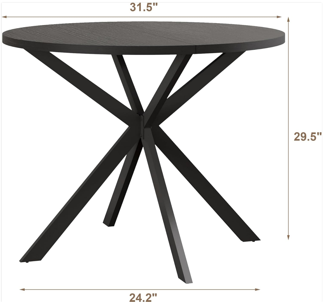
Dimensional diagram of the ChooChoo Round Dining Table.
