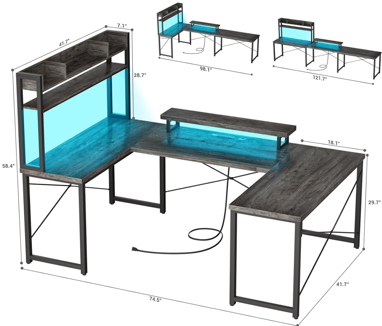
Image 3.1: Detailed dimensions of the desk in its U-shaped configuration, including height, width, and depth measurements. The desk measures approximately 75 inches in width, 41.7 inches in depth, and 58.41 inches in height (including the hutch). The working surface diagonal length is 86.6 inches.
