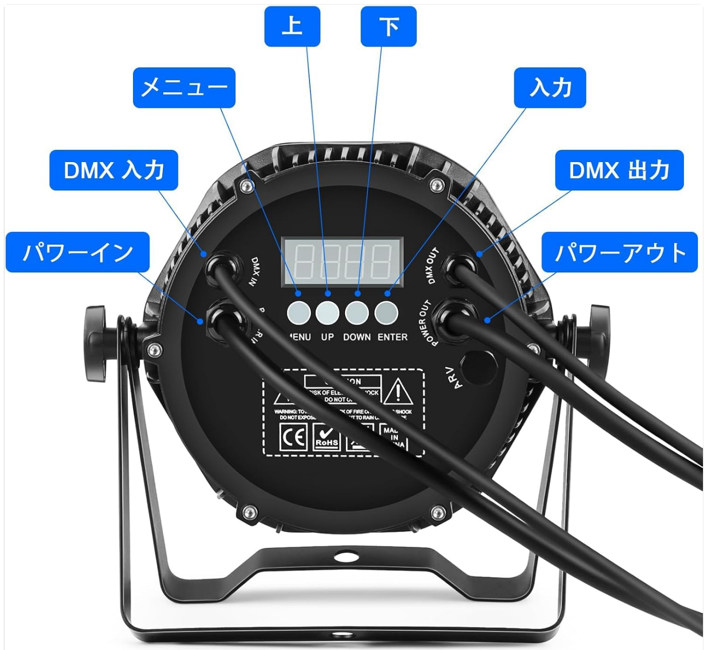
Image 5.3: The rear panel of the stage light, showing labeled ports for DMX IN, DMX OUT, POWER IN, and POWER OUT, along with control buttons (MENU, UP, DOWN, ENTER) and the digital display.
