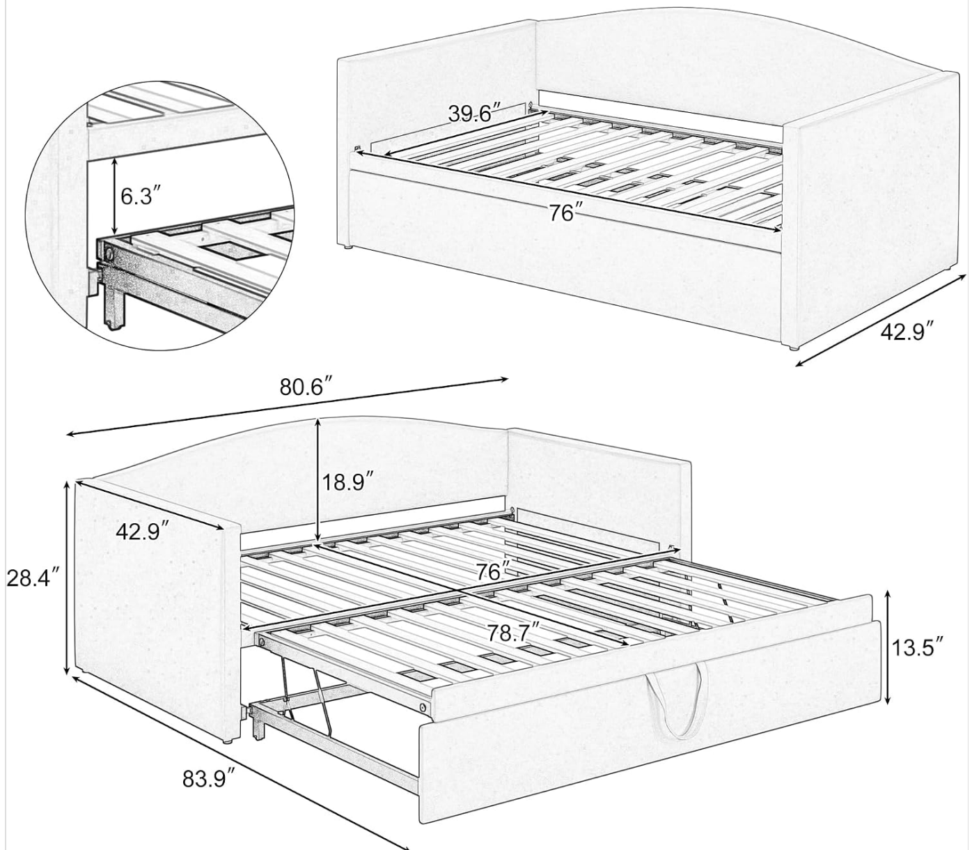
Image: Detailed dimension diagram for the Flieks Twin to King Daybed, showing measurements for both twin and extended king configurations.
