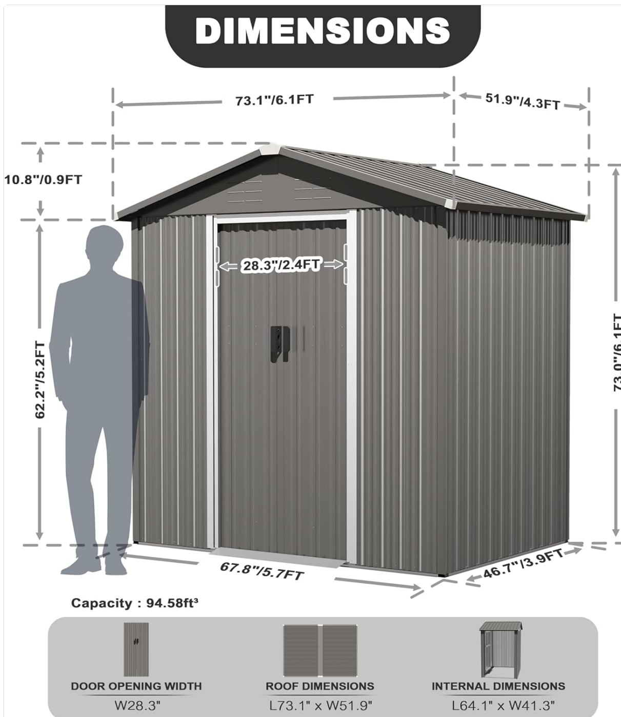
Image 7.1: Detailed dimensions of the NUU GARDEN Outdoor Storage Shed.
