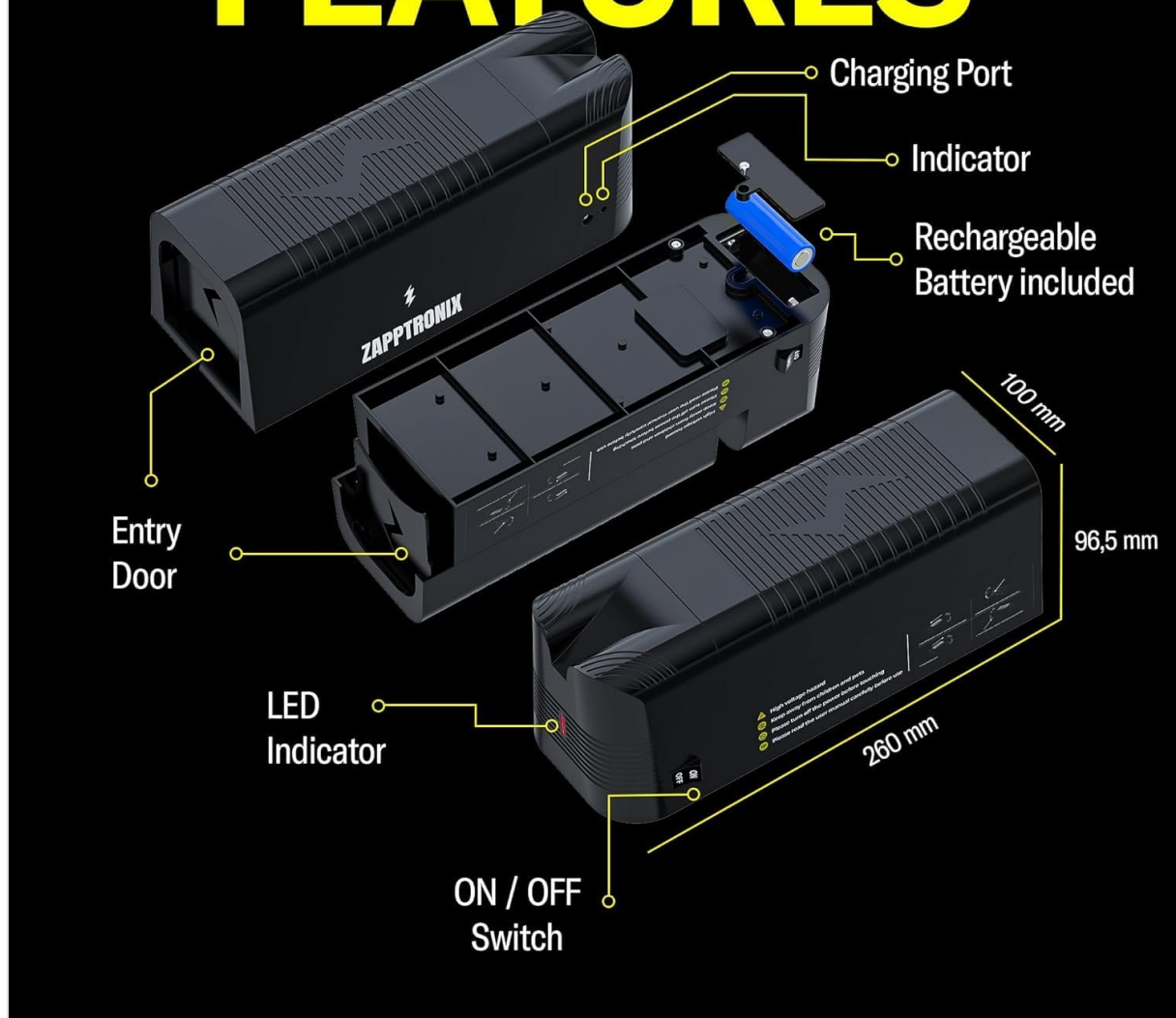
Image 4.1: Exploded view diagram of the ZAPPTRONIX Zapper highlighting its components: Charging Port, Indicator, Rechargeable Battery, Entry Door, LED Indicator, and ON/OFF Switch. Dimensions are also shown: 260mm length, 100mm width, 96.5mm height.
