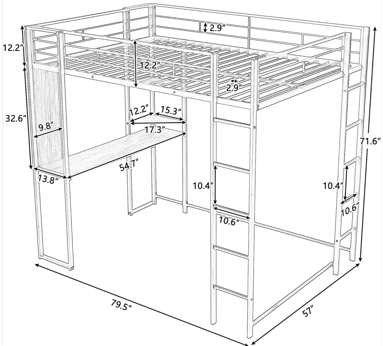
Image 7.1: Detailed dimensions of the loft bed components.
